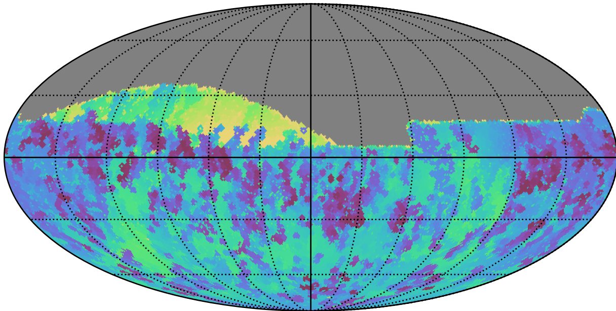
telescope_jerk_v3.5_10yrs Yr 1 all bands: Min skyBrightness
