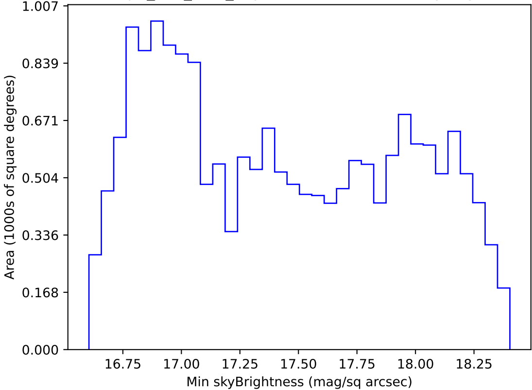
telescope_jerk_v3.5_10yrs WFD z band: Min skyBrightness
