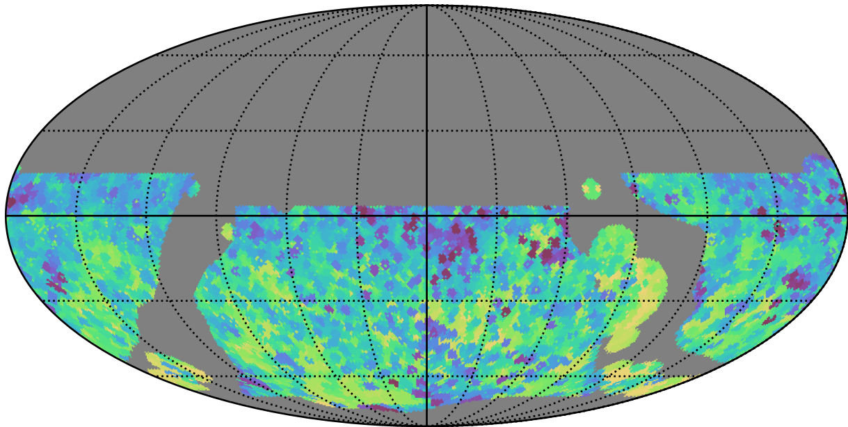
telescope_jerk_v3.5_10yrs WFD y band: Min skyBrightness
