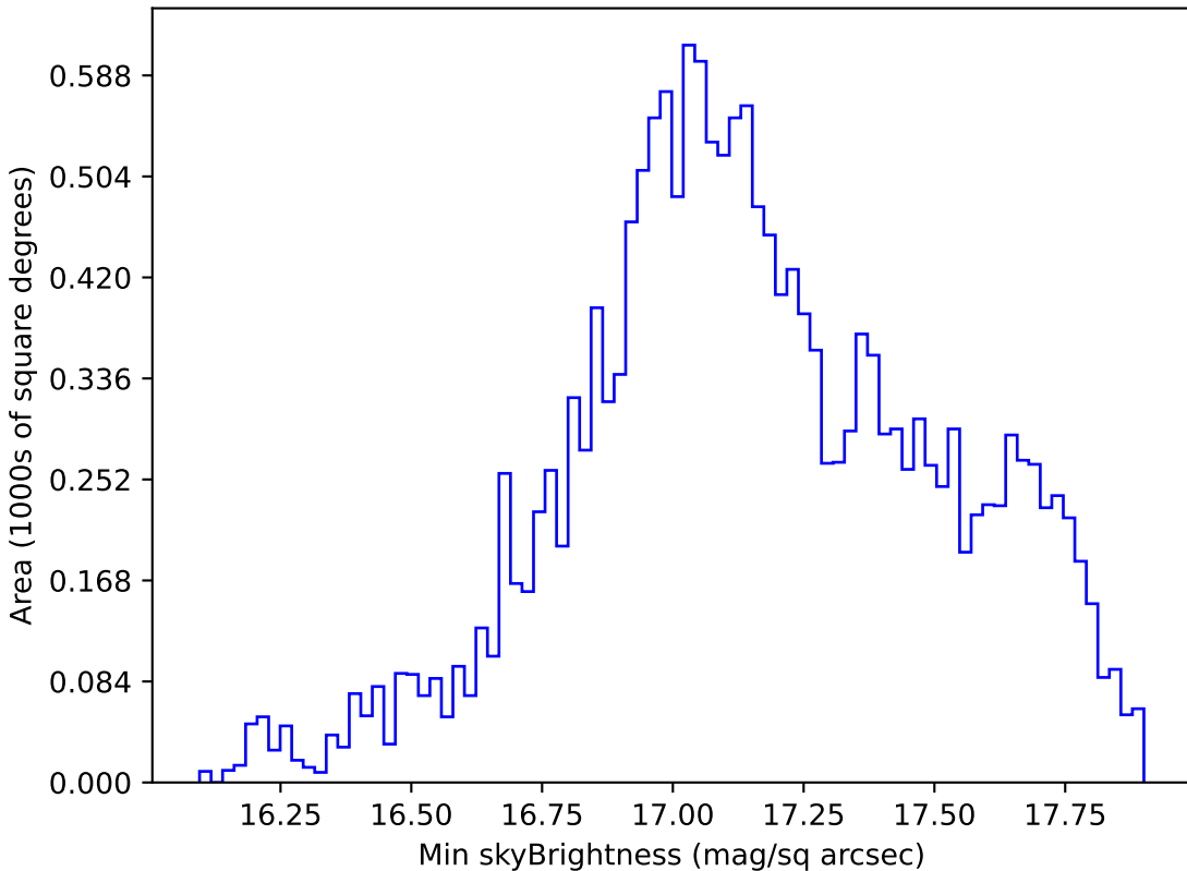
telescope_jerk_v3.5_10yrs WFD y band: Min skyBrightness
