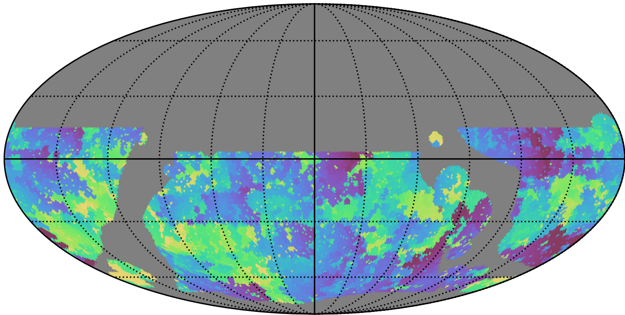
telescope_jerk_v3.5_10yrs WFD u band: Min skyBrightness
