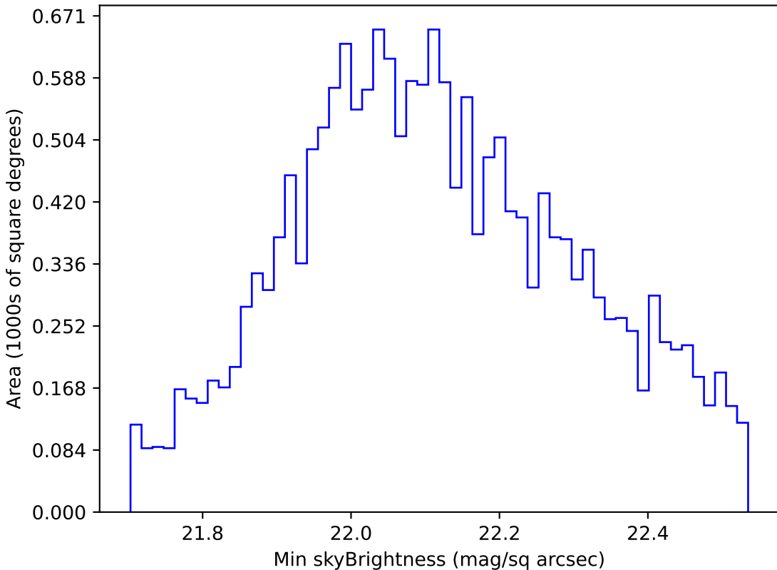
telescope_jerk_v3.5_10yrs WFD u band: Min skyBrightness
