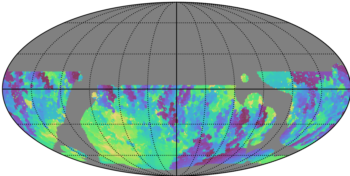
telescope_jerk_v3.5_10yrs WFD r band: Min skyBrightness
