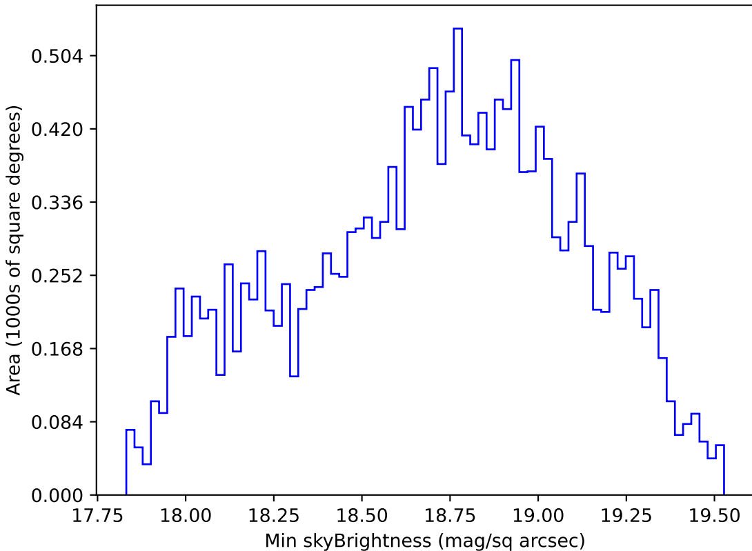
telescope_jerk_v3.5_10yrs WFD r band: Min skyBrightness
