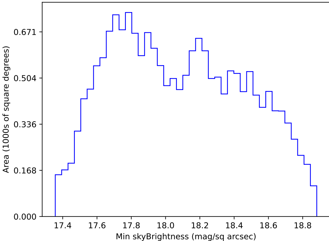
telescope_jerk_v3.5_10yrs WFD i band: Min skyBrightness
