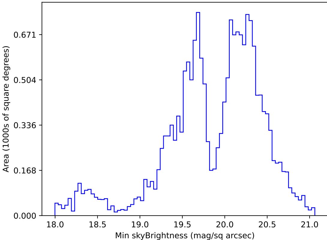
telescope_jerk_v3.5_10yrs WFD g band: Min skyBrightness
