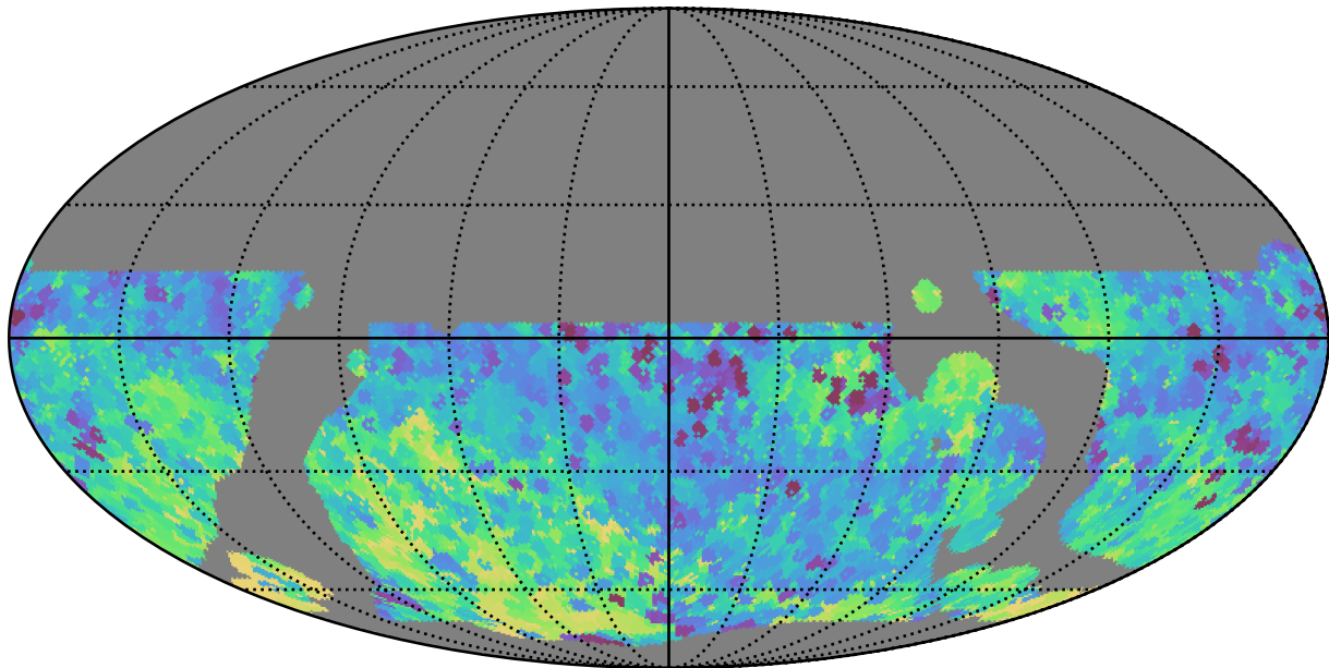
telescope_jerk_v3.5_10yrs WFD all bands: Min skyBrightness
