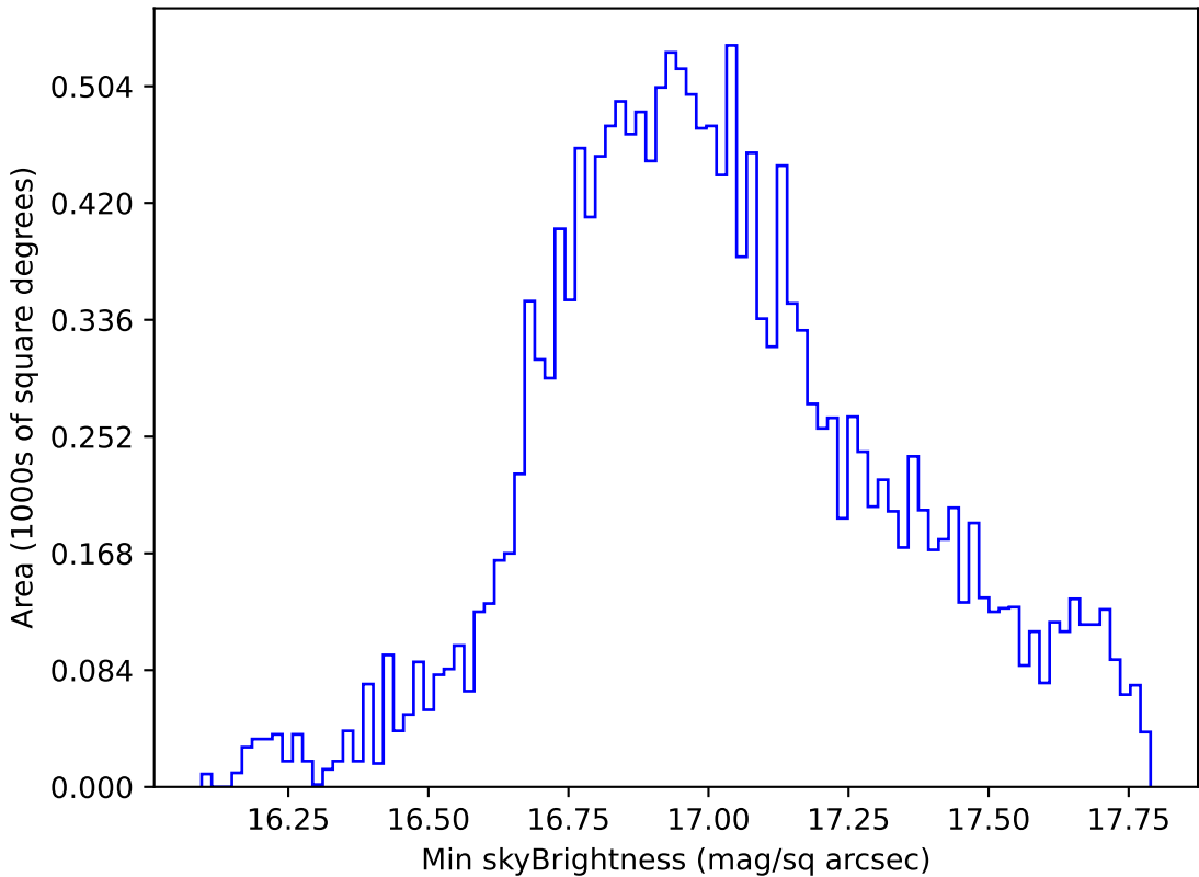
telescope_jerk_v3.5_10yrs WFD all bands: Min skyBrightness
