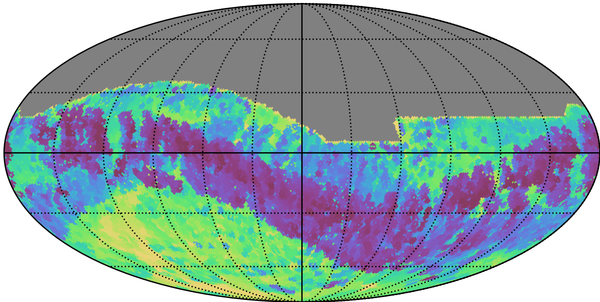
telescope_jerk_v3.5_10yrs All sky z band: Min skyBrightness
