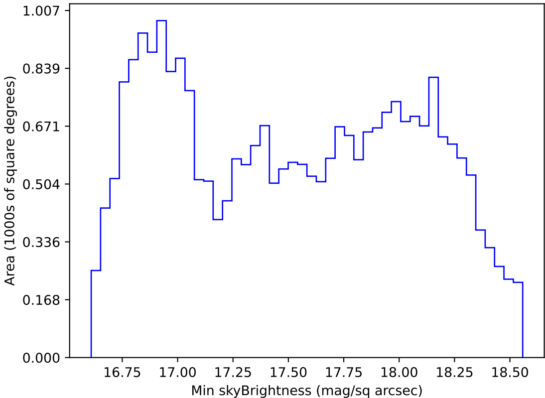
telescope_jerk_v3.5_10yrs All sky z band: Min skyBrightness
