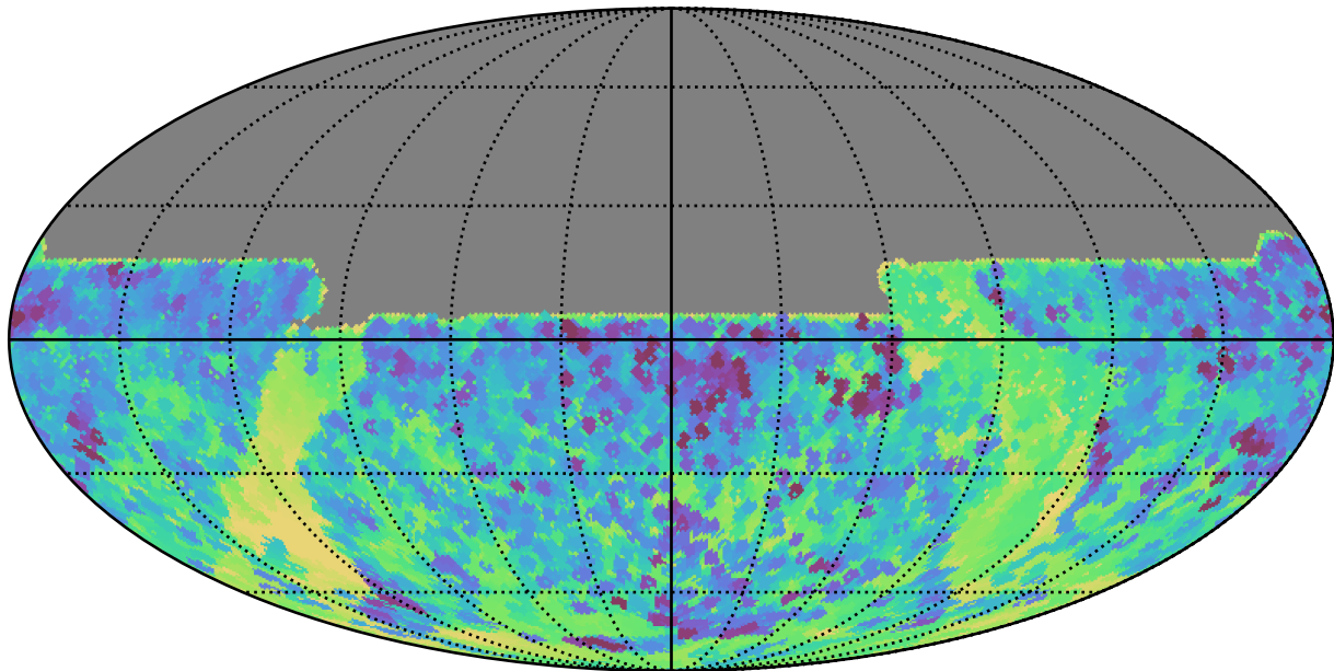
telescope_jerk_v3.5_10yrs All sky y band: Min skyBrightness
