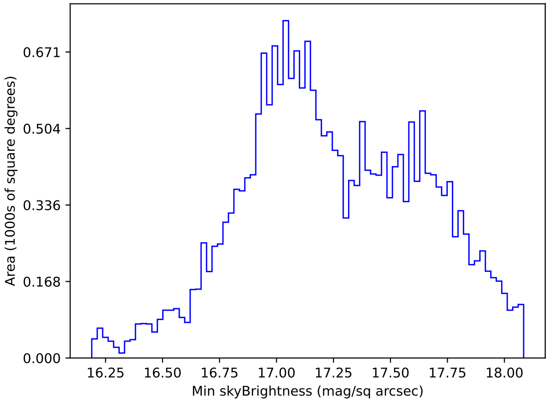
telescope_jerk_v3.5_10yrs All sky y band: Min skyBrightness
