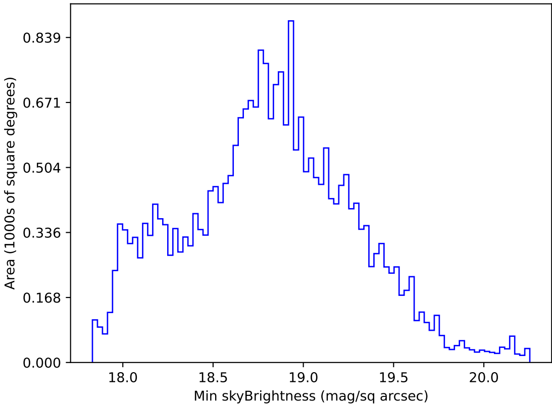
telescope_jerk_v3.5_10yrs All sky r band: Min skyBrightness
