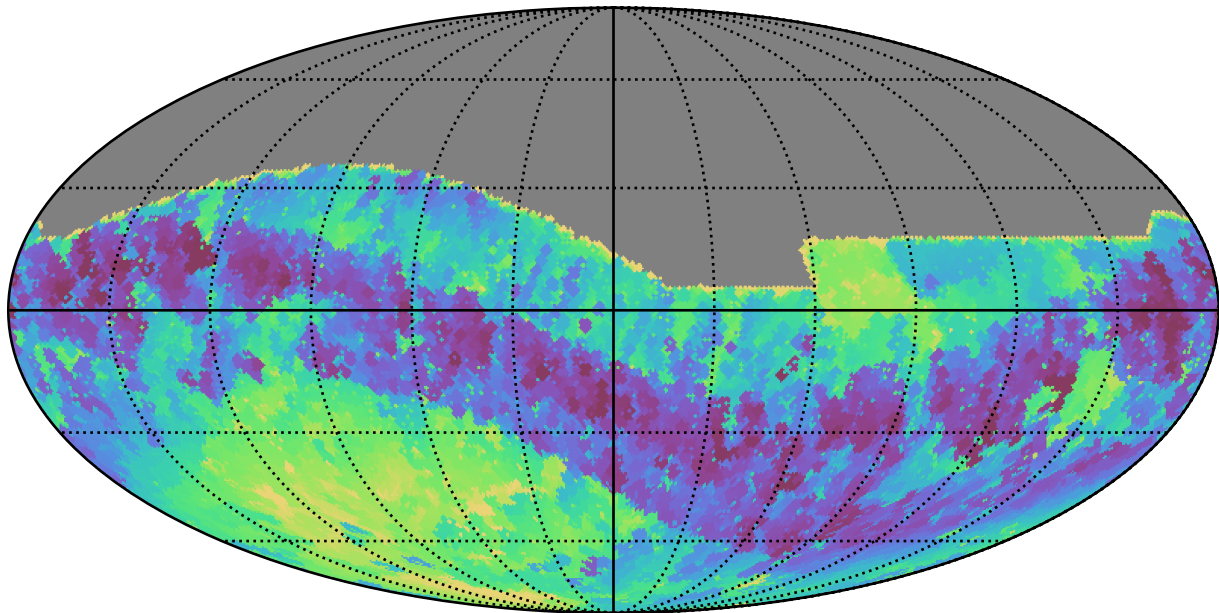
telescope_jerk_v3.5_10yrs All sky i band: Min skyBrightness
