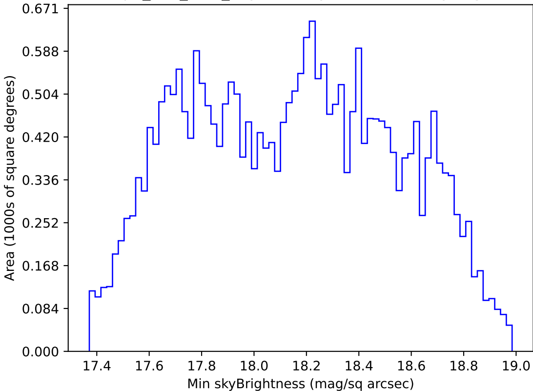
telescope_jerk_v3.5_10yrs All sky i band: Min skyBrightness
