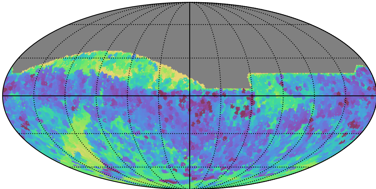
telescope_jerk_v3.5_10yrs All sky all bands: Min skyBrightness
