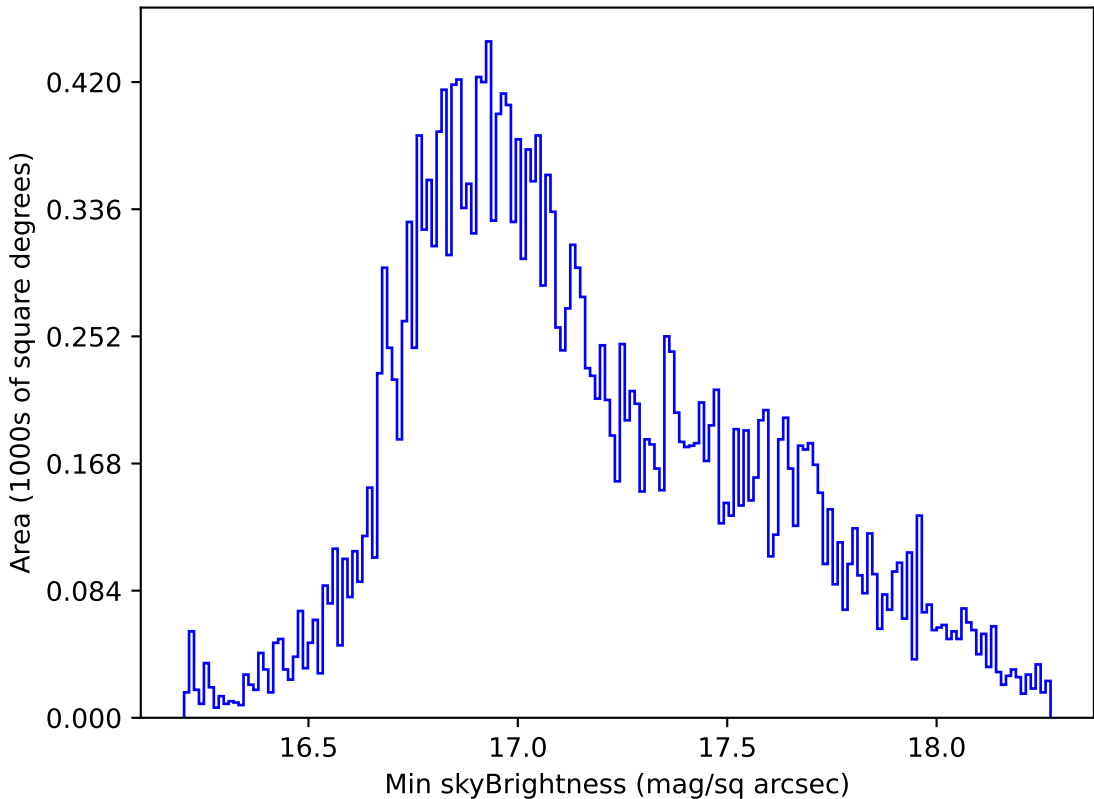
telescope_jerk_v3.5_10yrs All sky all bands: Min skyBrightness
