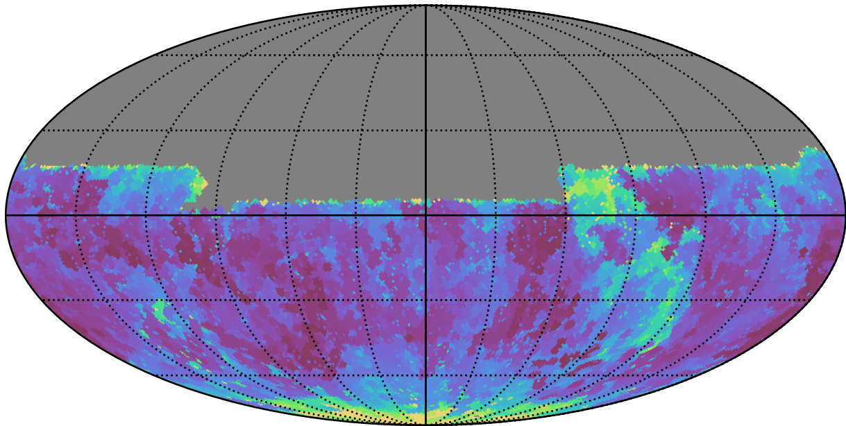
telescope_jerk_v3.5_10yrs Yr 1 y band: Min seeingGeom
