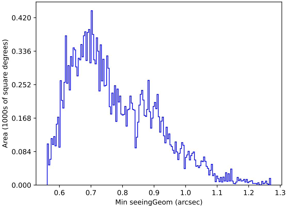
telescope_jerk_v3.5_10yrs Yr 1 u band: Min seeingGeom
