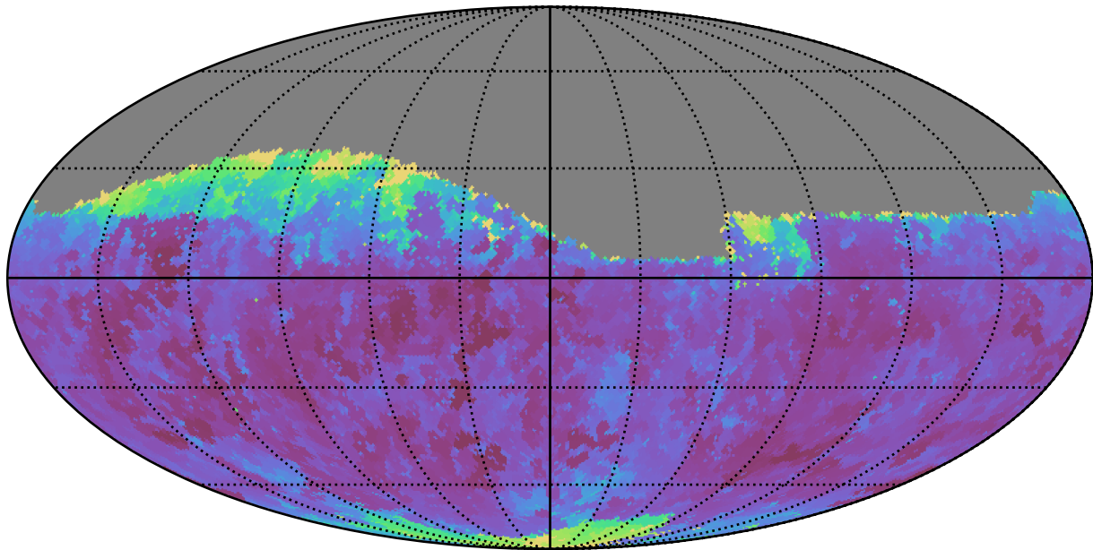
telescope_jerk_v3.5_10yrs Yr 1 r band: Min seeingGeom
