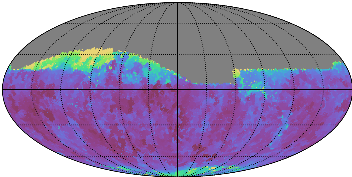
telescope_jerk_v3.5_10yrs Yr 1 i band: Min seeingGeom
