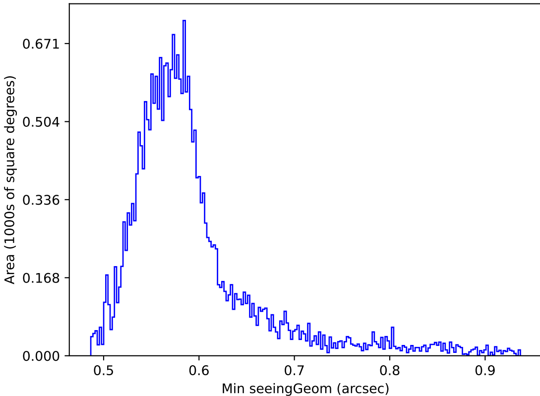
telescope_jerk_v3.5_10yrs Yr 1 all bands: Min seeingGeom
