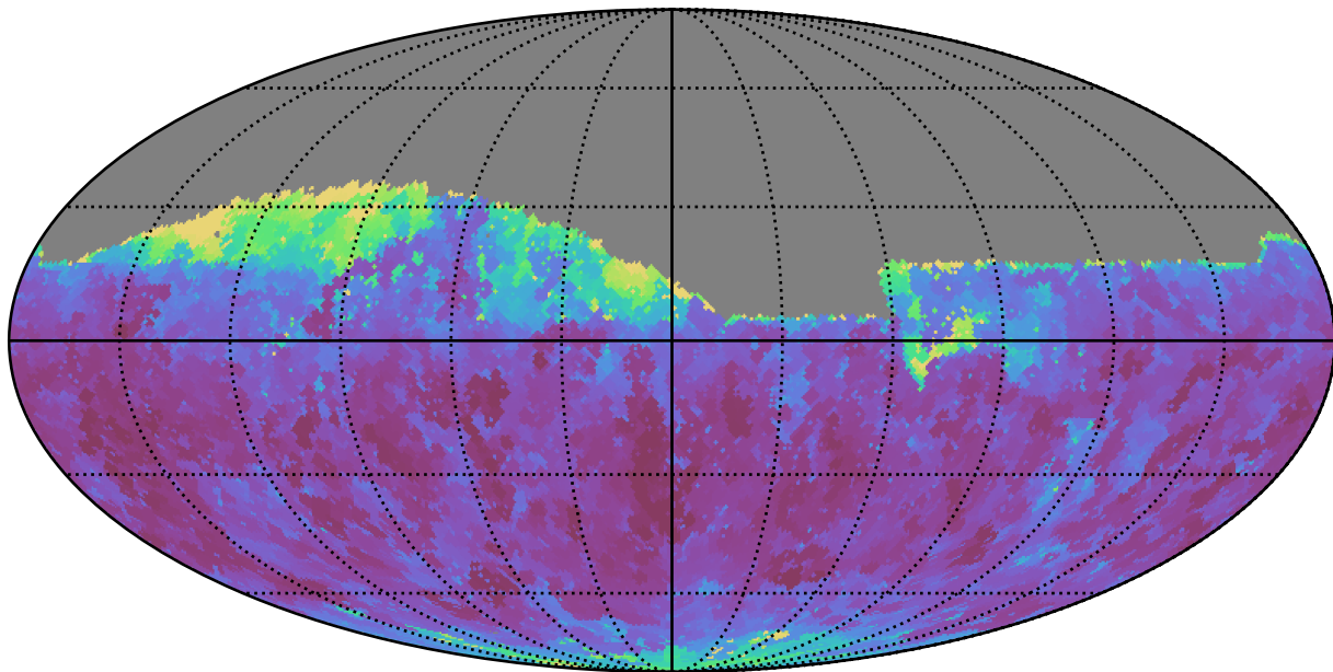
telescope_jerk_v3.5_10yrs Yr 1 z band: Min seeingEff
