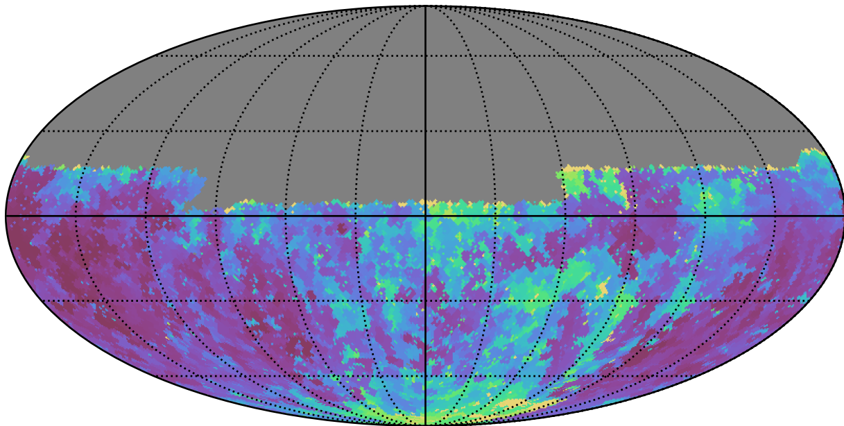
telescope_jerk_v3.5_10yrs Yr 1 u band: Min seeingEff
