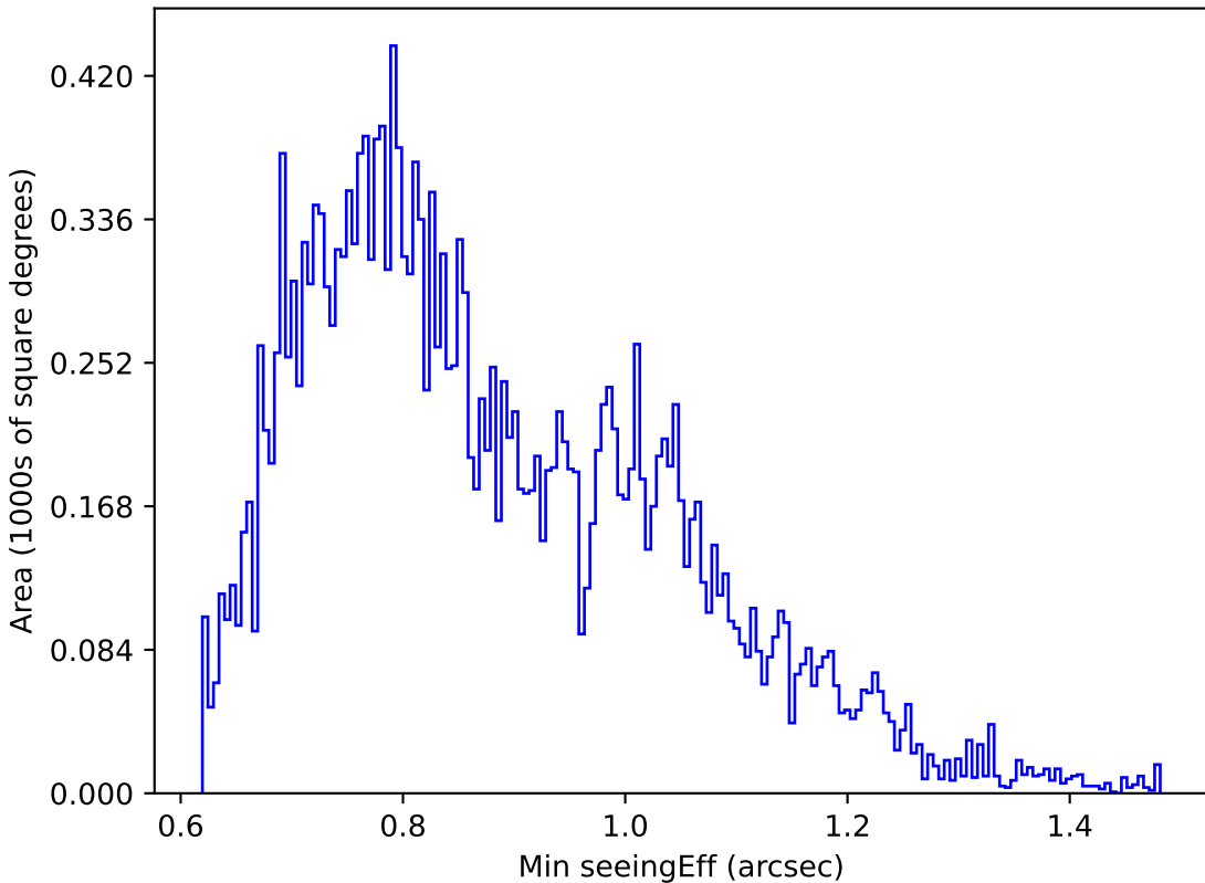
telescope_jerk_v3.5_10yrs Yr 1 u band: Min seeingEff
