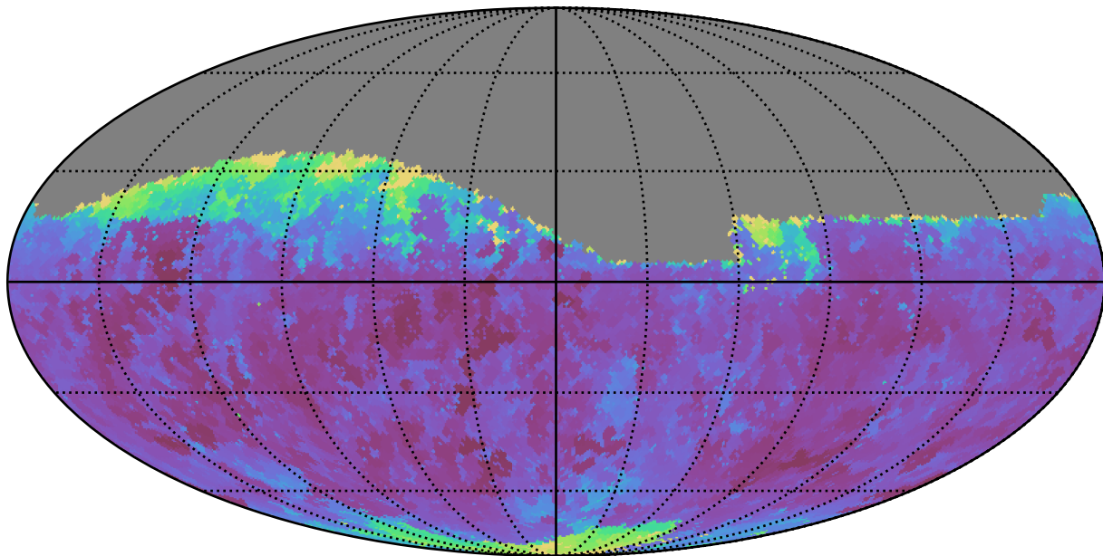
telescope_jerk_v3.5_10yrs Yr 1 r band: Min seeingEff
