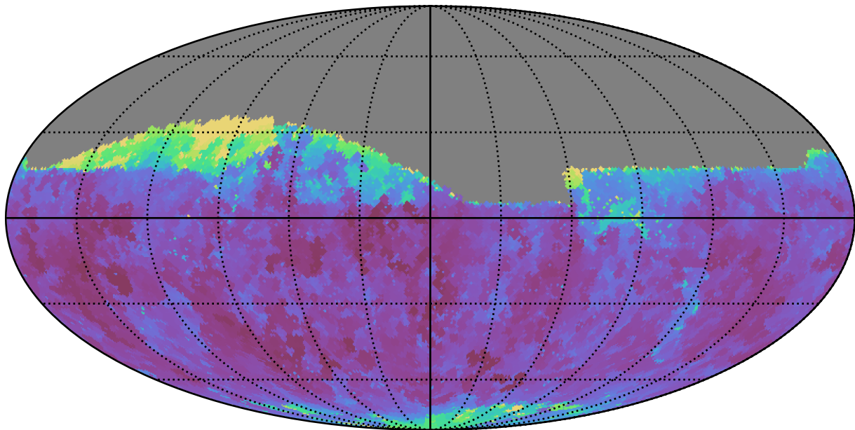
telescope_jerk_v3.5_10yrs Yr 1 i band: Min seeingEff
