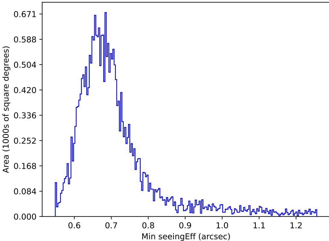
telescope_jerk_v3.5_10yrs Yr 1 i band: Min seeingEff
