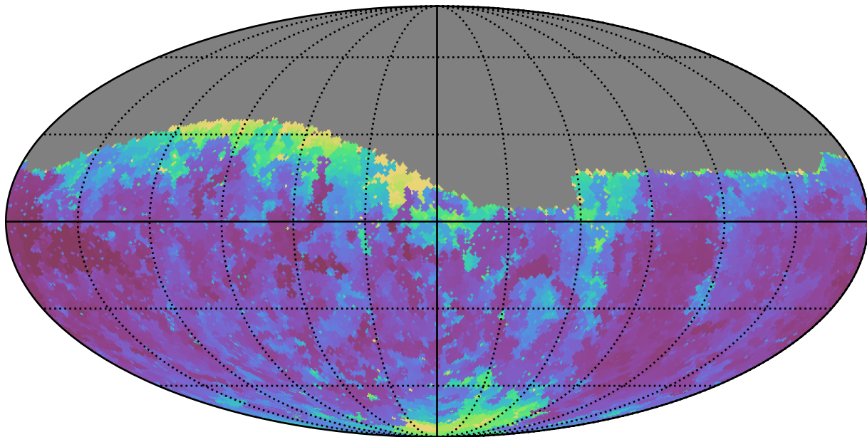
telescope_jerk_v3.5_10yrs Yr 1 g band: Min seeingEff
