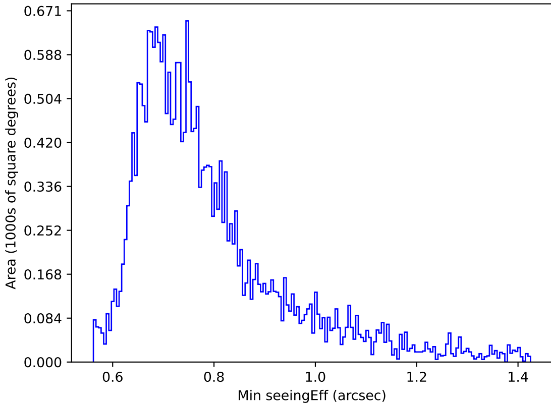
telescope_jerk_v3.5_10yrs Yr 1 g band: Min seeingEff
