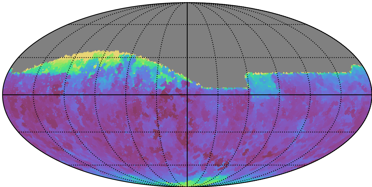
telescope_jerk_v3.5_10yrs Yr 1 all bands: Min seeingEff
