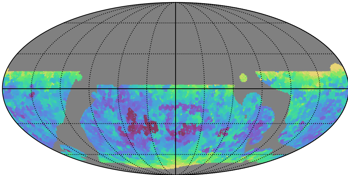
telescope_jerk_v3.5_10yrs WFD z band: Min seeingEff
