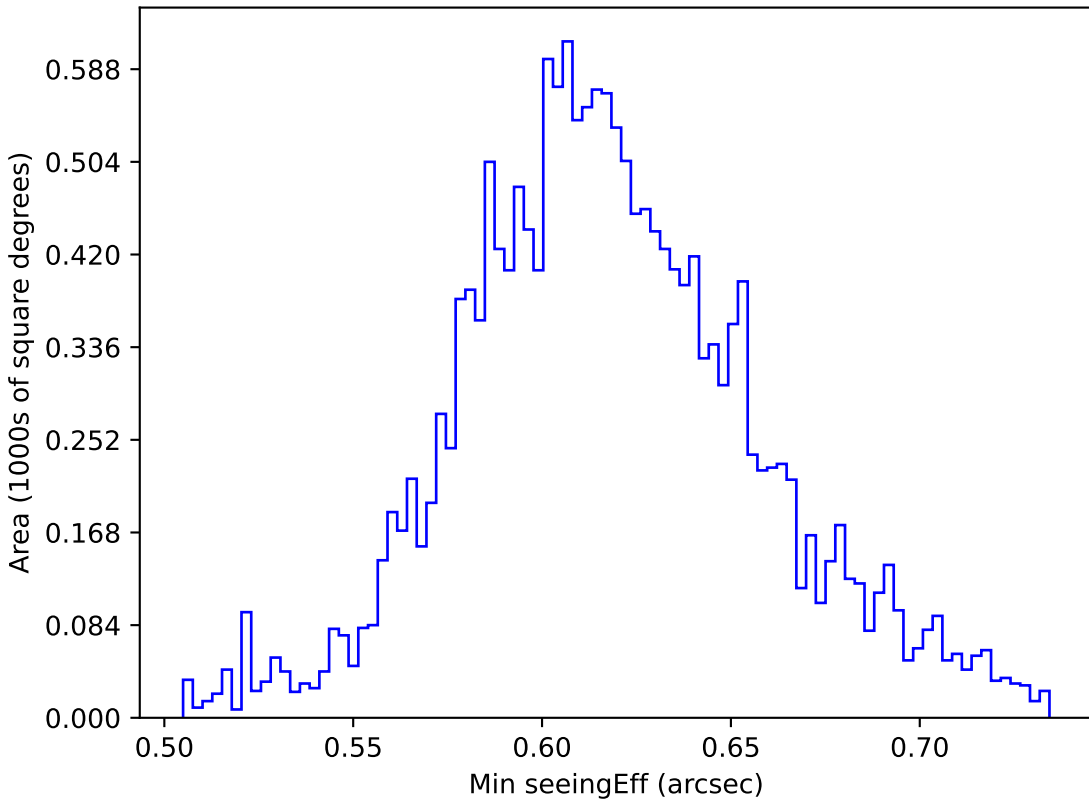
telescope_jerk_v3.5_10yrs WFD z band: Min seeingEff
