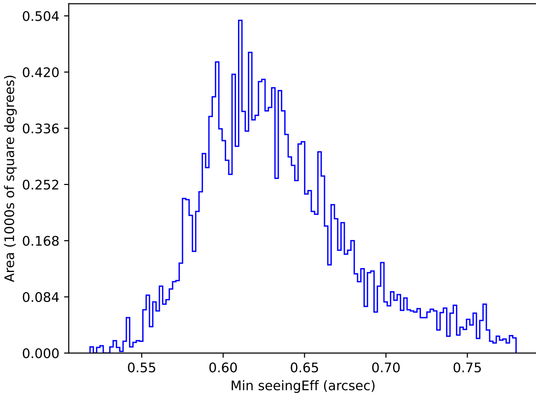
telescope_jerk_v3.5_10yrs WFD y band: Min seeingEff
