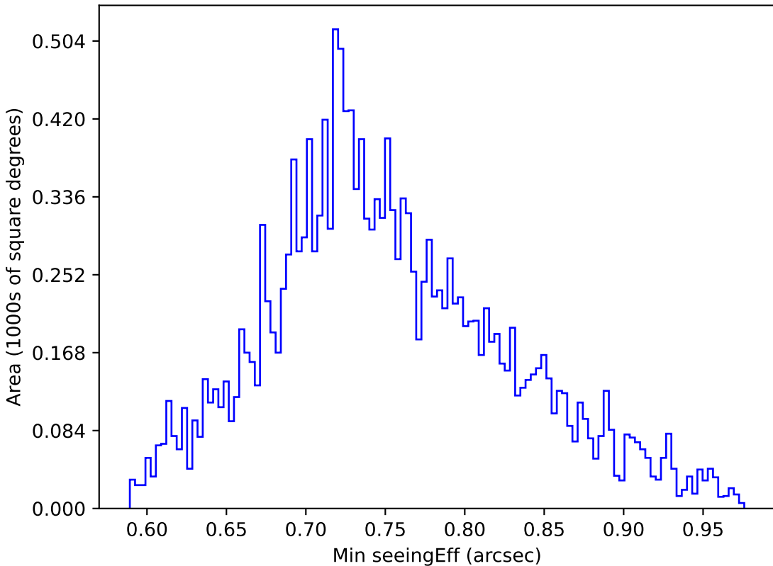
telescope_jerk_v3.5_10yrs WFD u band: Min seeingEff
