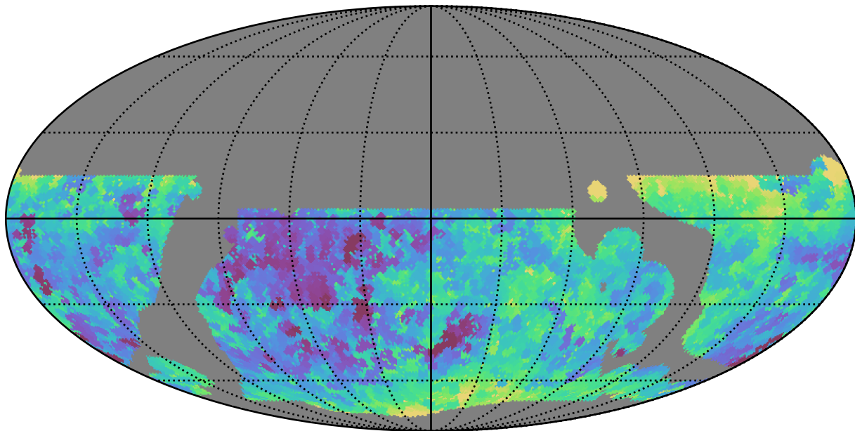
telescope_jerk_v3.5_10yrs WFD r band: Min seeingEff
