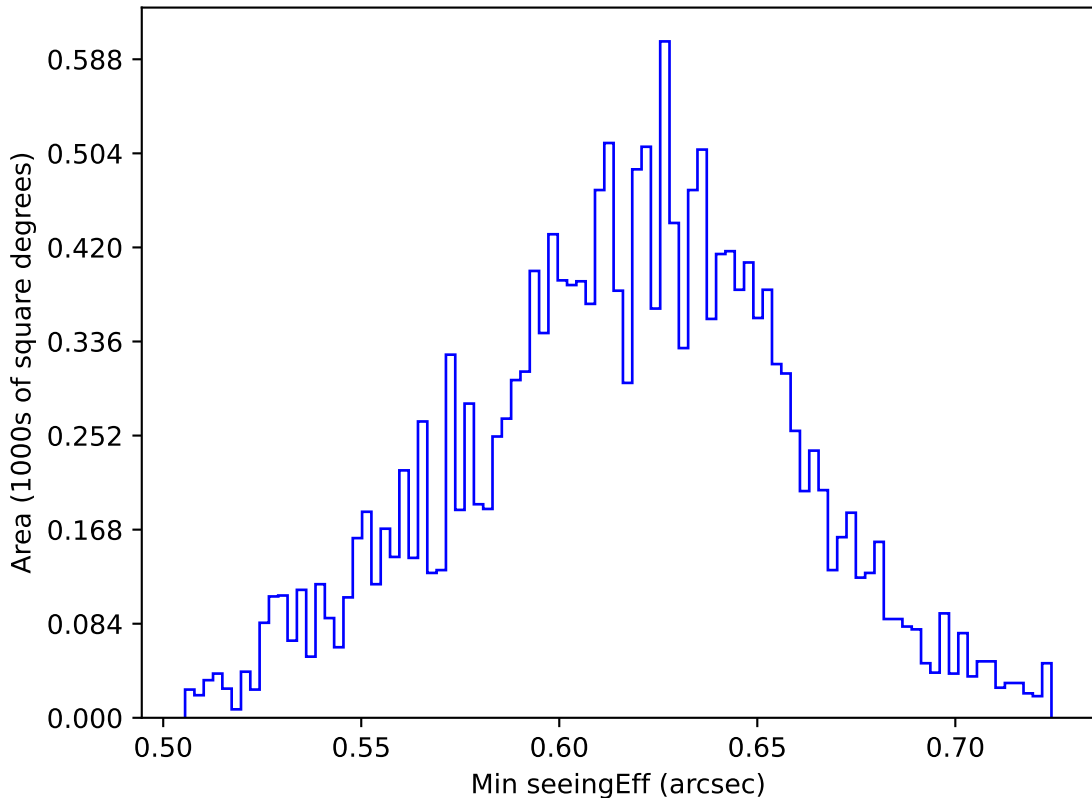
telescope_jerk_v3.5_10yrs WFD r band: Min seeingEff
