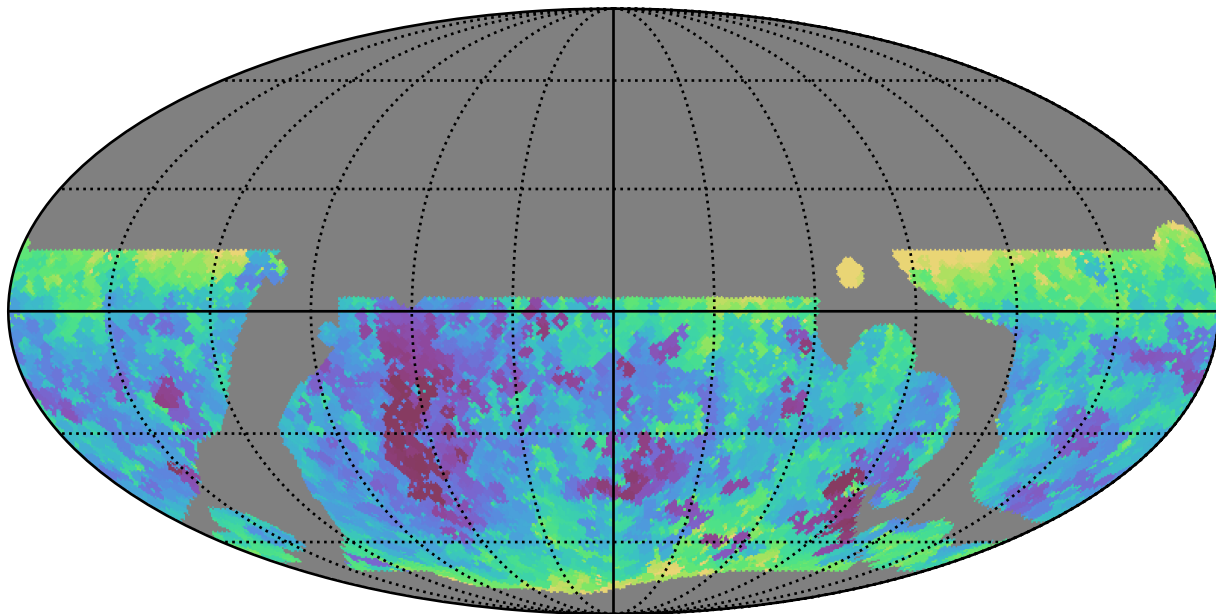
telescope_jerk_v3.5_10yrs WFD i band: Min seeingEff
