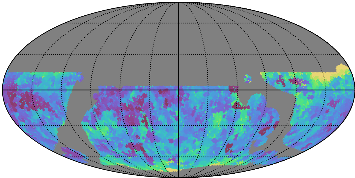
telescope_jerk_v3.5_10yrs WFD g band: Min seeingEff
