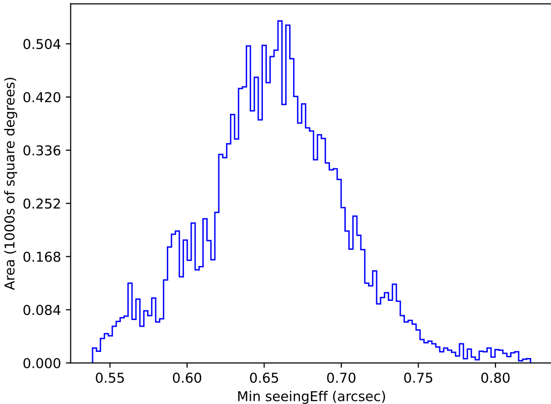
telescope_jerk_v3.5_10yrs WFD g band: Min seeingEff
