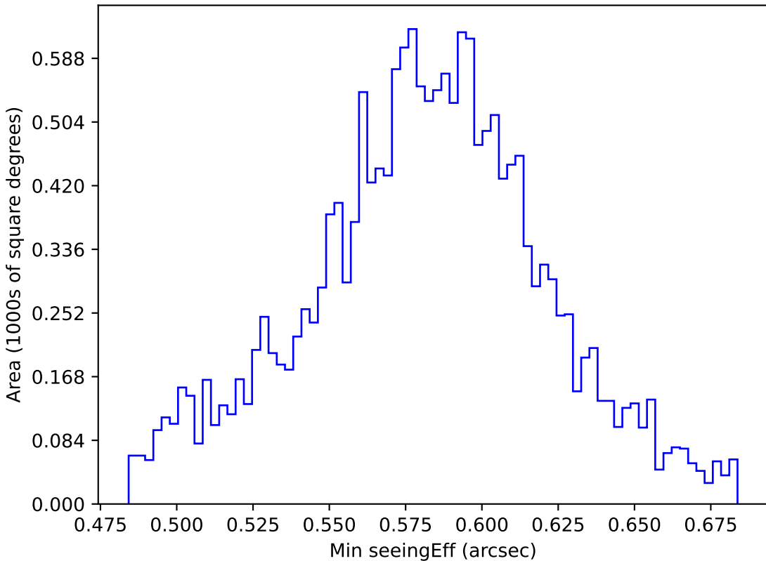
telescope_jerk_v3.5_10yrs WFD all bands: Min seeingEff
