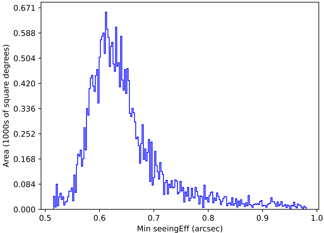
telescope_jerk_v3.5_10yrs All sky z band: Min seeingEff
