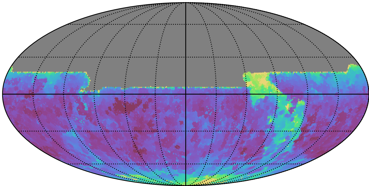
telescope_jerk_v3.5_10yrs All sky y band: Min seeingEff
