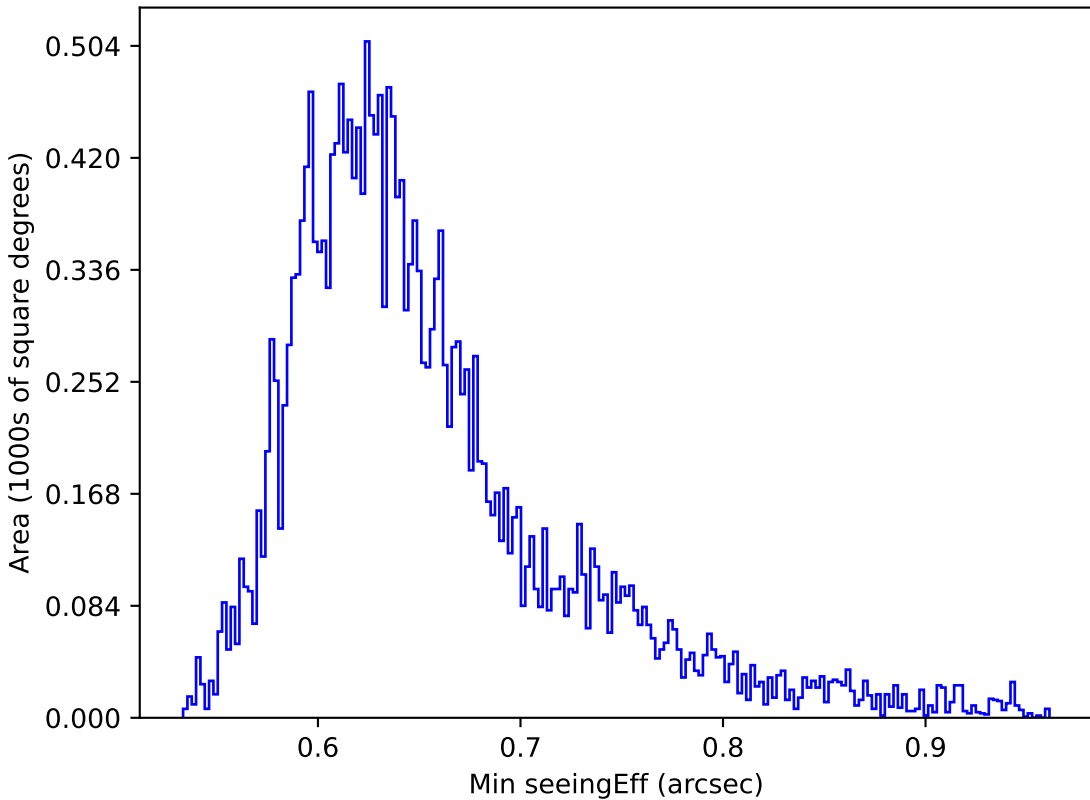
telescope_jerk_v3.5_10yrs All sky y band: Min seeingEff
