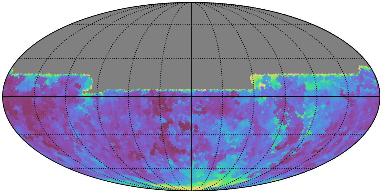
telescope_jerk_v3.5_10yrs All sky u band: Min seeingEff
