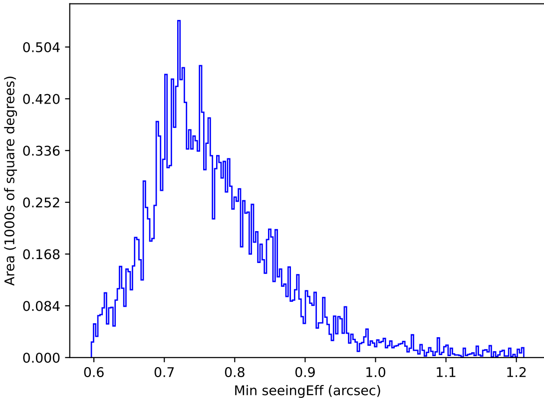
telescope_jerk_v3.5_10yrs All sky u band: Min seeingEff
